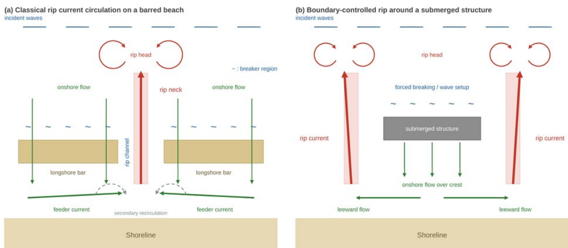
Figure 2. Schematic of rip current circulation: (a) classical bar-channel rip system with feeder currents, rip neck and rip head, including the secondary recirculation cells near the shoreline; (b) boundary-controlled rip currents around a submerged structure driven by wave setup over the crest.
