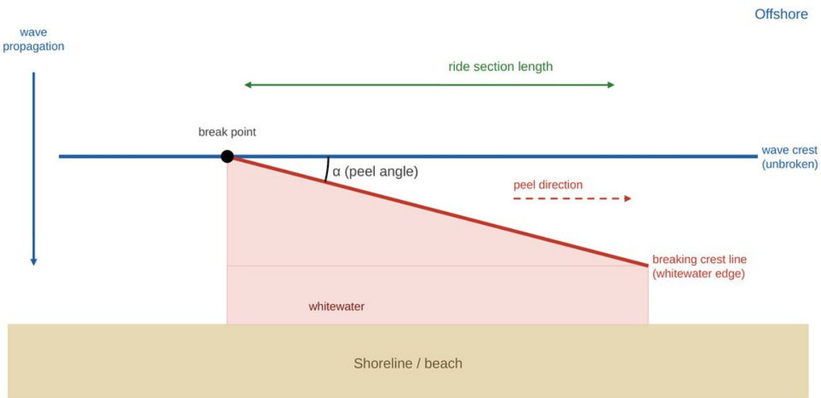
Figure 1. Geometric definition of surfing wave parameters. The peel angle \alpha is defined between the unbroken wave crest and the breaking crest line (whitewater edge), and the ride section length is determined by the along-crest breaking speed.
